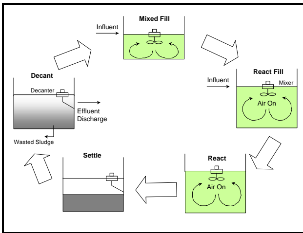
FIGURE 3 SBR SEQUENCE OF OPERATION
