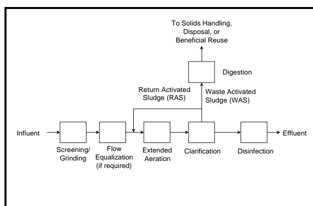
FIGURE 1 PROCESS FLOW DIAGRAM FOR A TYPICAL EXTENDED AERATION PLANT
